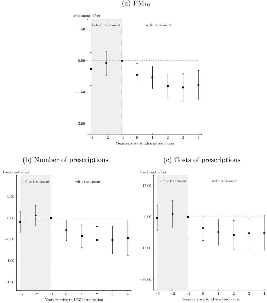
Figure A.3: Event-study Estimates Excluding the Never Treated
