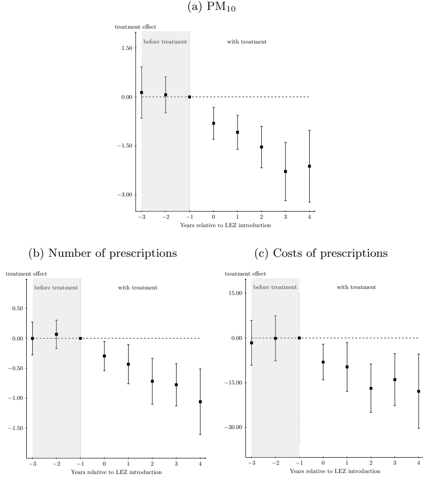
Figure A.1: Event-study Estimates of LEZ Effects - Excluding All Already Treated Counties from the Control Group
