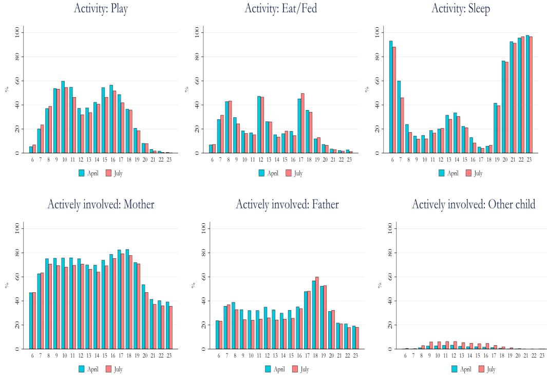
Figure 2: Time-use diaries
