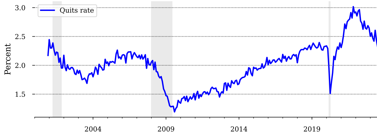
Figure 10: Quits rate
